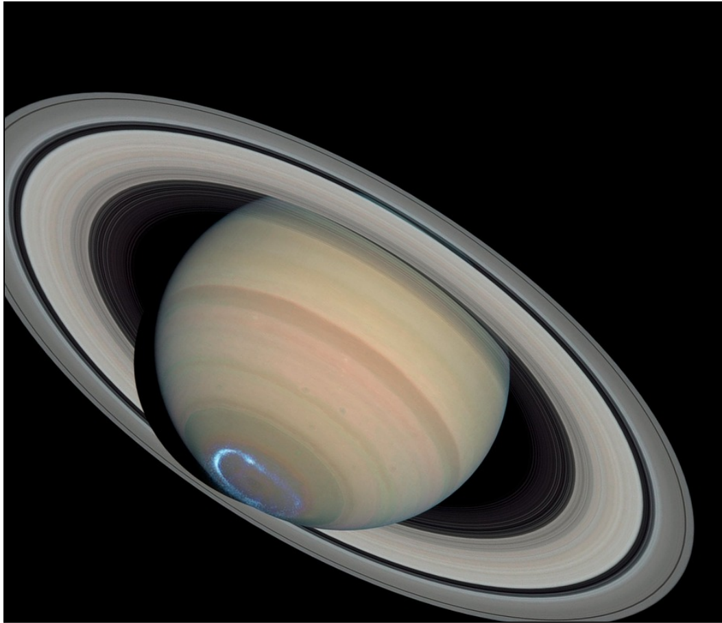
Saturn
